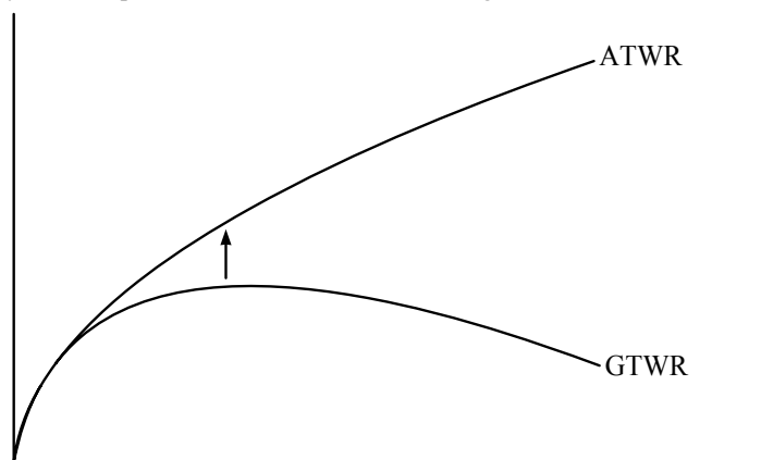
Figure 7-3 The efficient frontier with/without reinvestment
