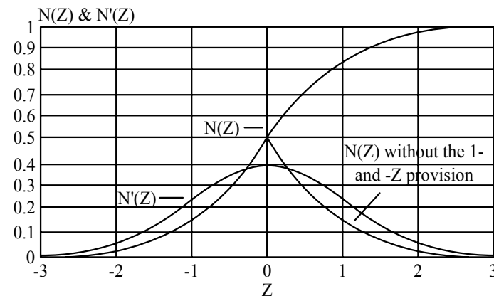
Figure 3-9 Doing away with the 1- and -Z provision in Equation (3.21).
