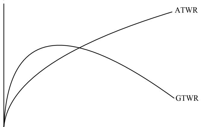
Figure 7-4 The efficient frontier with/without reinvestment.
